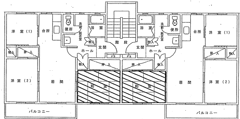
国設宿舎(3LK) S=1/X
