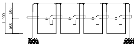
No.3油分離槽 S=1:70
