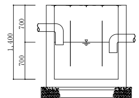
No.11油分離槽 S=1:70
