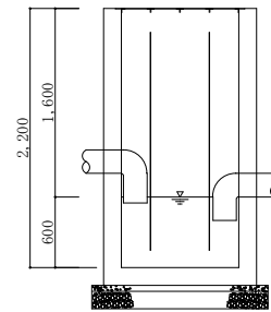
No.5, No.7油分離槽 S=1:70
