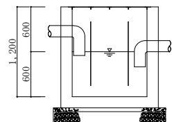
No.1, No.2油分離槽 S=1:70
