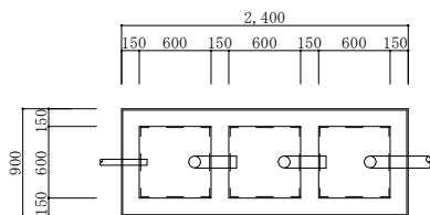
No.1, No.2油分離槽 S=1:70
