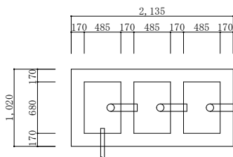
No.3油分離槽 S=1:70
