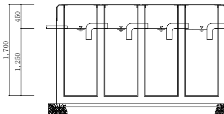
No.4油分離槽 S=1:70
