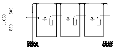
No.6油分離槽 S=1:70
