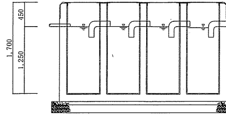
No.4油分離槽 S=1:70
