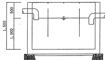
No.9油分離槽 S=1:70
