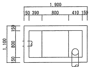
No.9油分離槽 S=1:70
