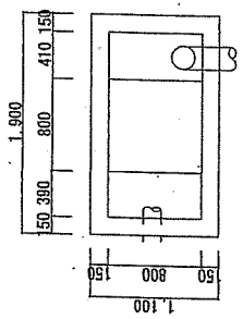
No.9油分離槽 S=1:70
