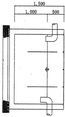
No.9油分離槽 S=1:70
