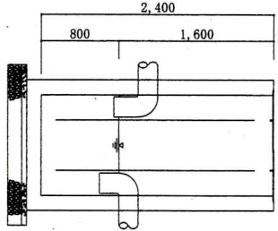
No.4油分離槽 S=1:70
