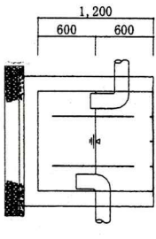
No.1, No.2油分離槽 S=1:70
