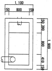
No.9油分離槽 S=1:70
