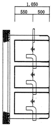
No.6油分離槽 S=1:70
