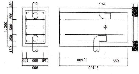
No.5油分離槽 S=1:70
