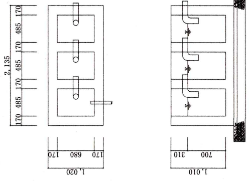
No.9油分離槽 S=1:70
