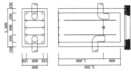
No.1油分離槽 S=1:70
