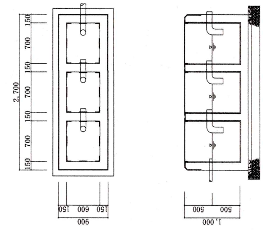
No.4油分離槽 S=1:70
