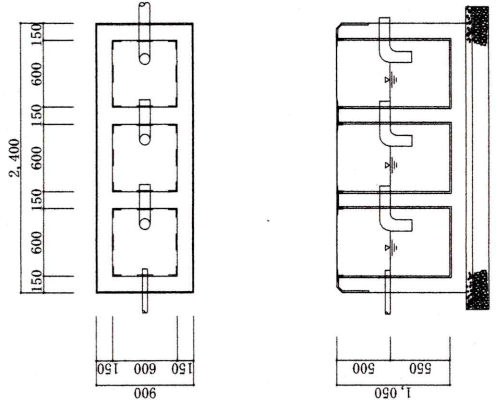
No.7油分離槽 S=1:70
