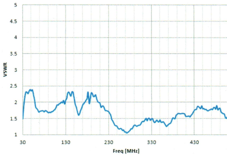
Antenna with 10m coaxial cable.
