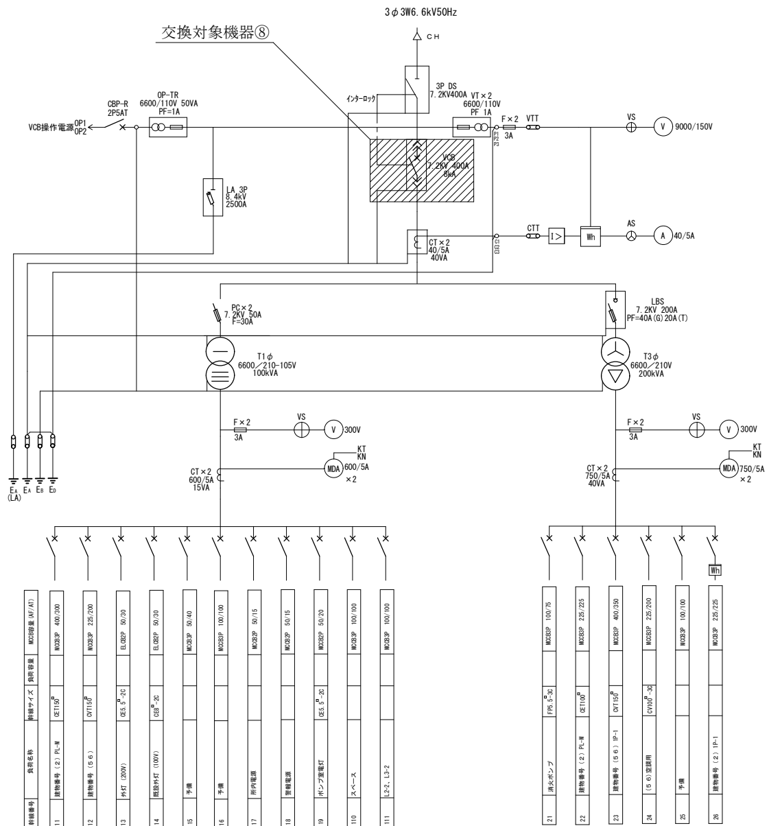
図8.1-単線結線図 (No.1 1)
