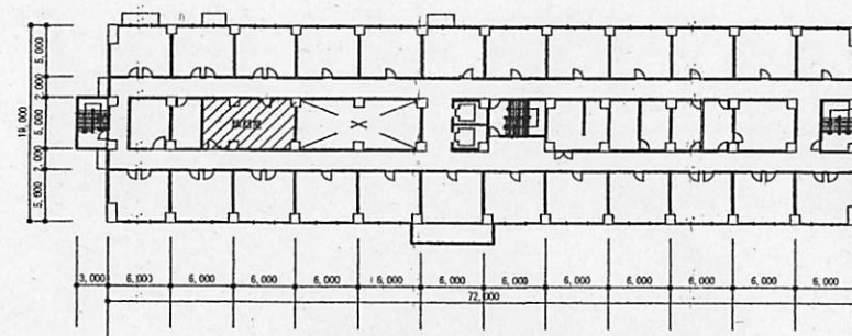
④第2隊舎2～8階平面図S=1:800
