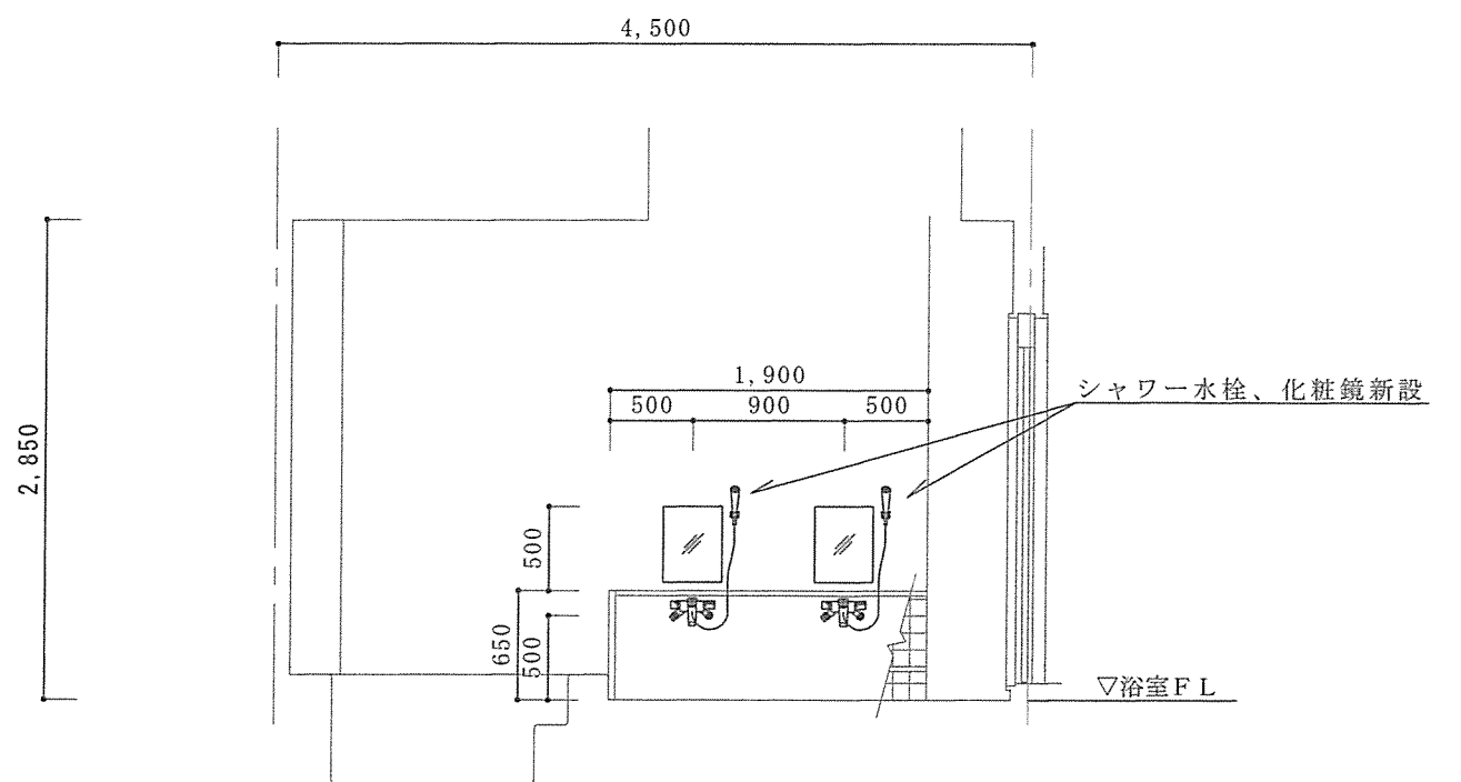
浴場展開図A面改修前 S=1/50
